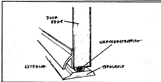
Figure 6. Exterior Door weather stripping
