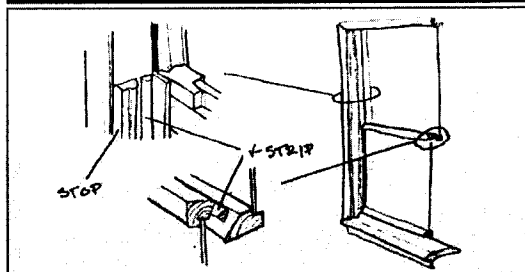
Figure 5. Window weather stripping
