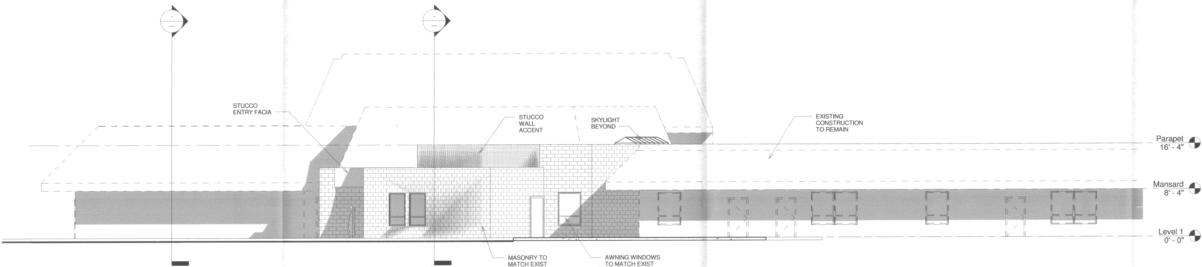
② East 1/8" = 1'-0"
