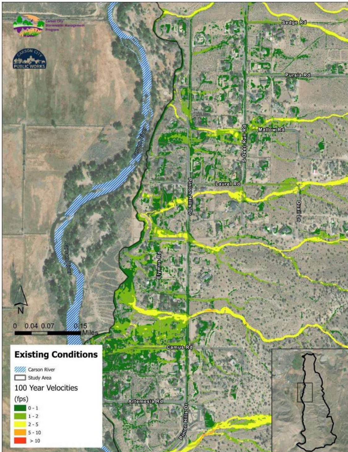
Figure 3-7: Existing Conditions 100-year Velocities
