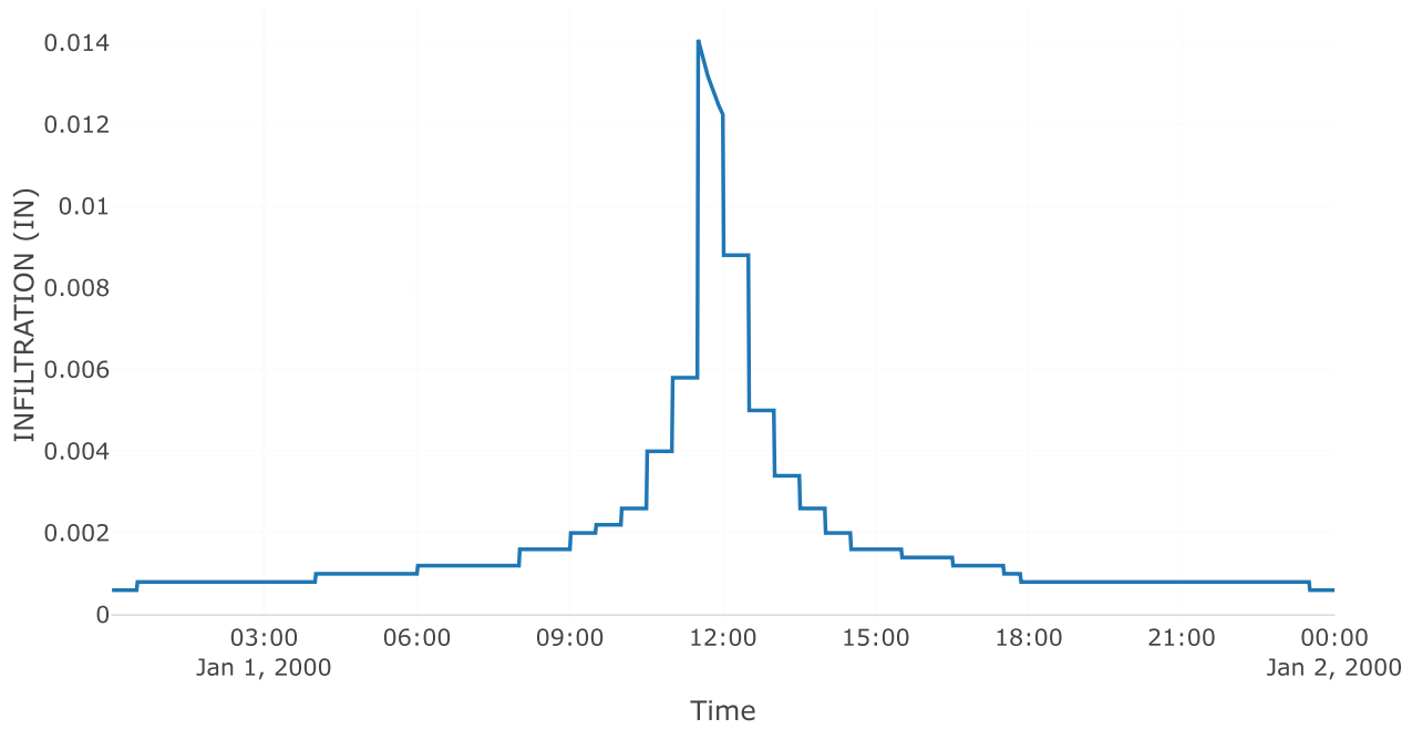
Soil Infiltration
