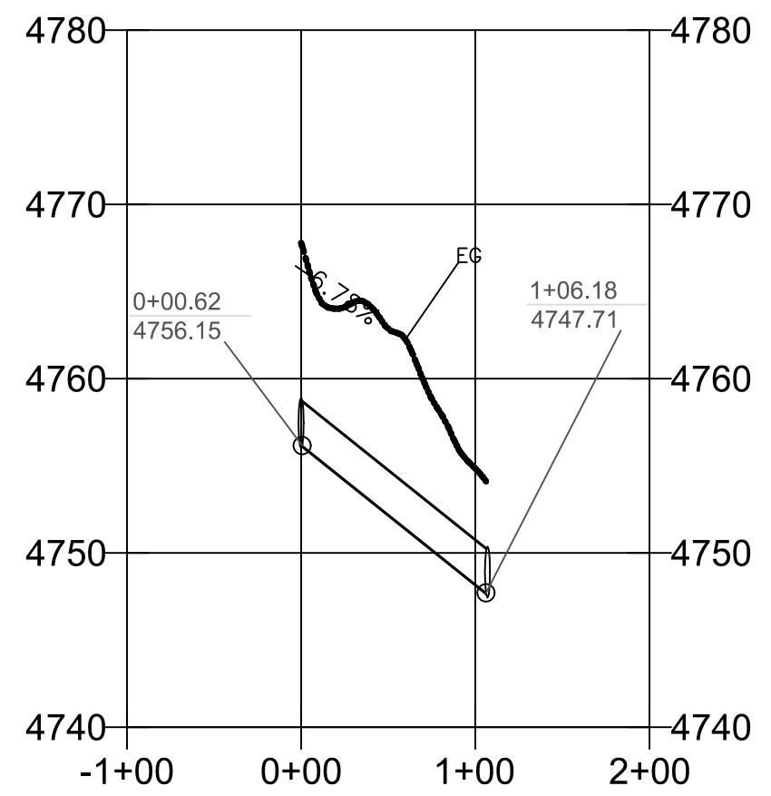
30-Inch HDPE Culvert
