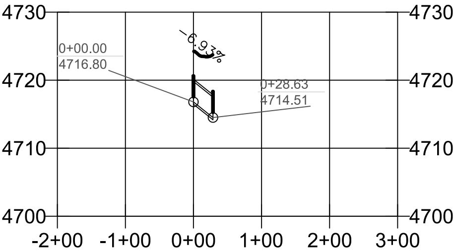
(W) 36-Inch RCP Culvert w/ Headwalls
