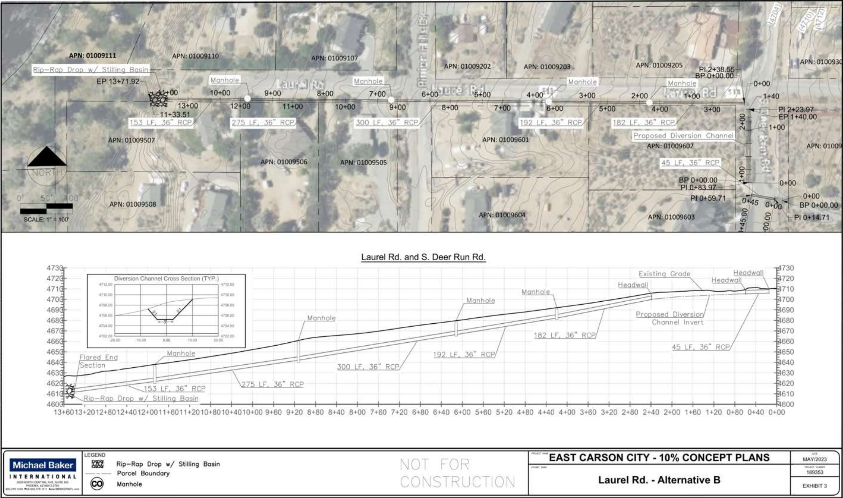
Figure 6-5: Proposed Concept Design Laurel Road Alternative B
