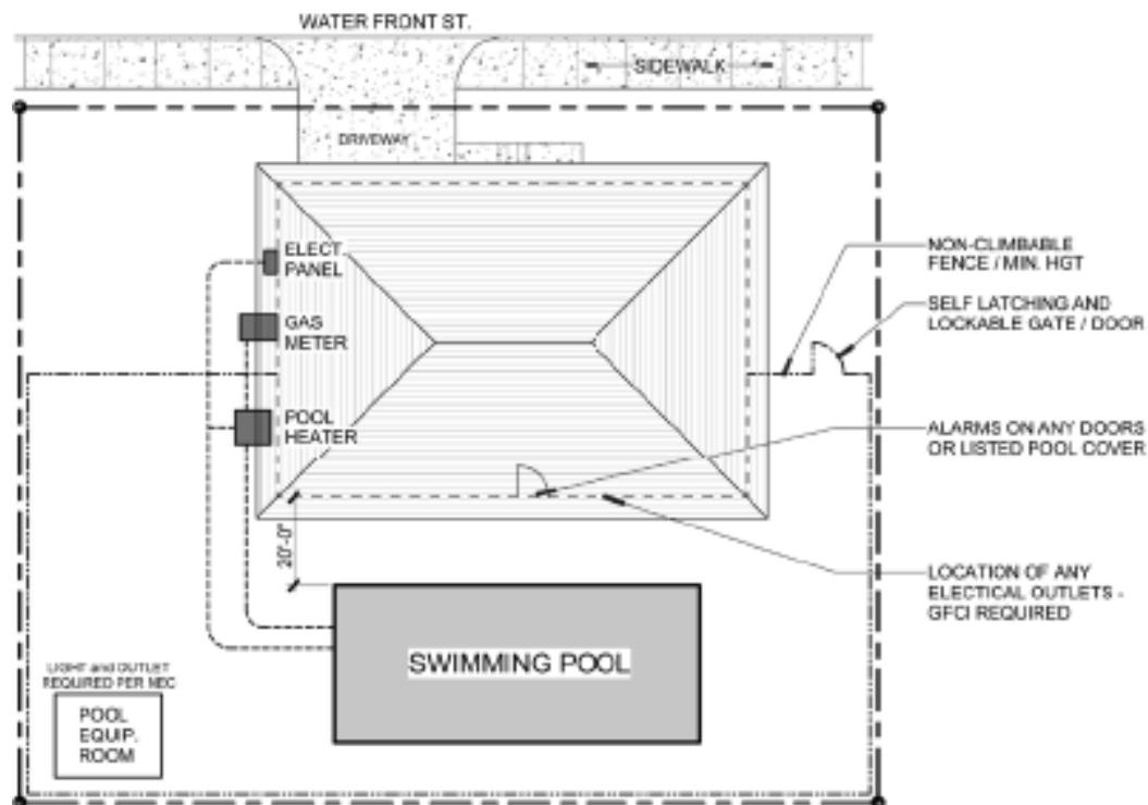
SWIMMING POOL SITE PLAN
